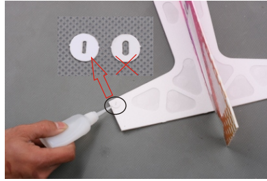
11. Install the round doublers to the pre-reserved holes (4 places) on the horizontal stabilizer.
