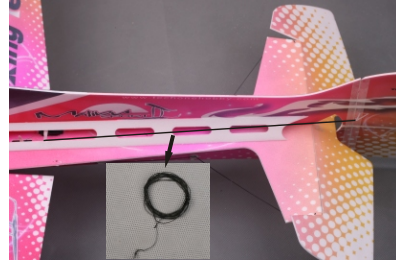
38. Link the servos and rudder control horns with threads. Make sure the threads are taut and the two ends of the servo arms are tied with threads.
