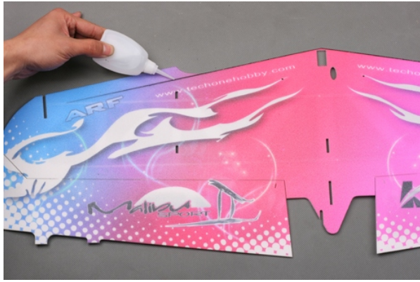
3. Glue 2pcs carbon fiber strips on the front of wing with some foam-friendly C/A.
