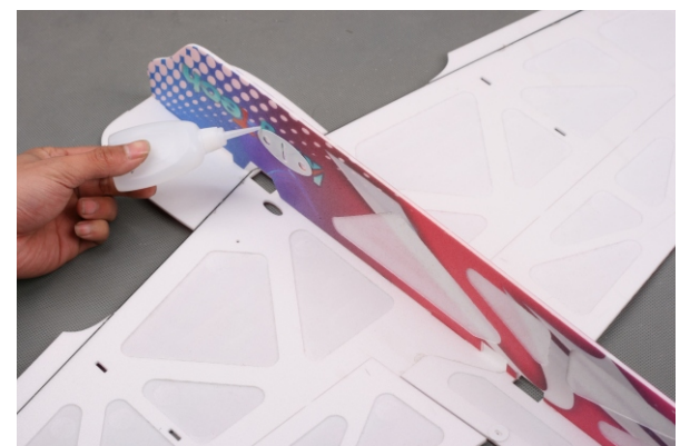
8. Install the landing gear reinforcements.
