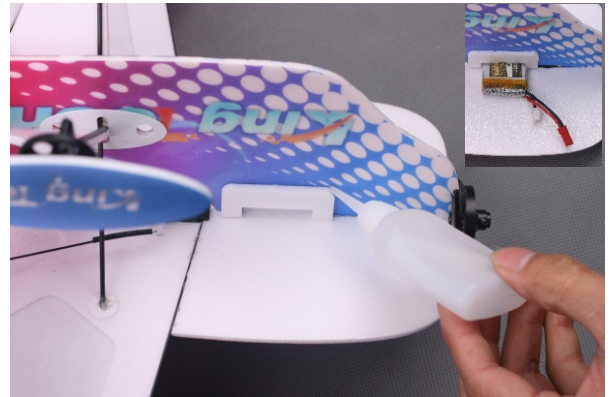
45. Place the strengthened foam slices around the pre-reserved battery hole and use some foam friendly C/A to fix. Then insert the battery into the battery hole.
