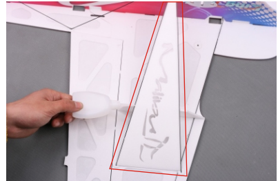
18. Apply some C/A to all the joints of carbon fiber rods and the wing strengthen foam.
