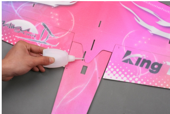
5. Key the rear of horizontal fuselage into the wing and apply some foam-friendly C/A.
