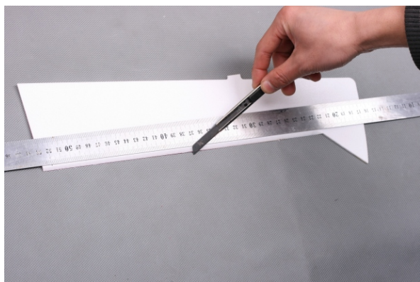
1. Cut 45° bevel on the two ailerons.
