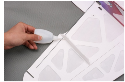
12. Insert the wing fence into the pre-reserved slot of the middle wing and apply some foam friendly C/A.
