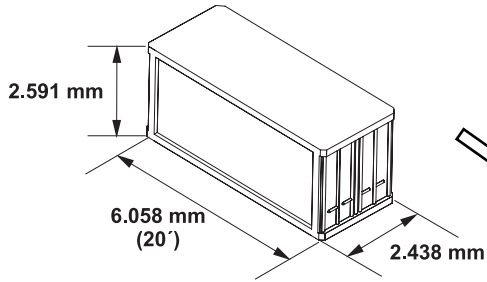
20' Standard General Purpose Container
