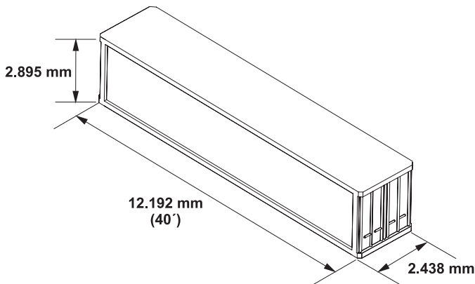
40' Standard High Cube General Purpose Container
