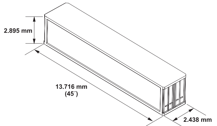
45' Standard High Cube General Purpose Container
