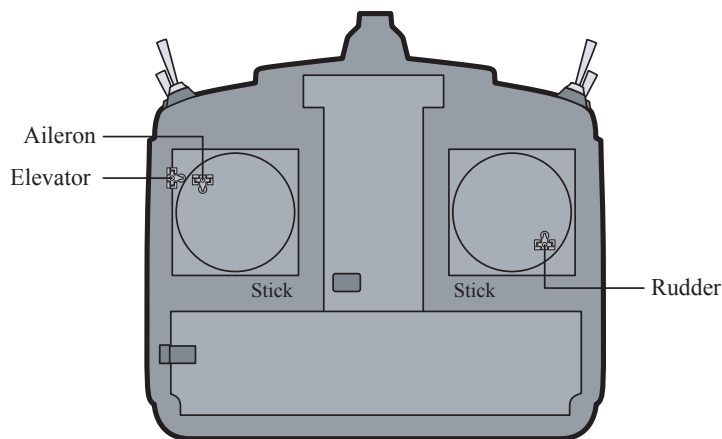
Mode 2 transmitter with rear cover removed.
